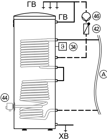
Vitocell 100-B
